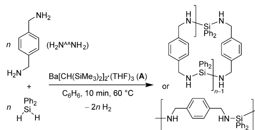
Scheme 1. Dehydropolymerization of \text{Ph}_2\text{SiH}_2 and \text{H}_2\text{N}^{\wedge}\text{NH}_2 catalyzed by A .
